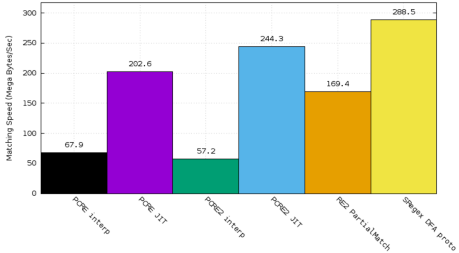
Benchmarking regex /\s[a-zA-Z]{0,12}\s/ matching file mtent12.txt of size 19.1 MB
